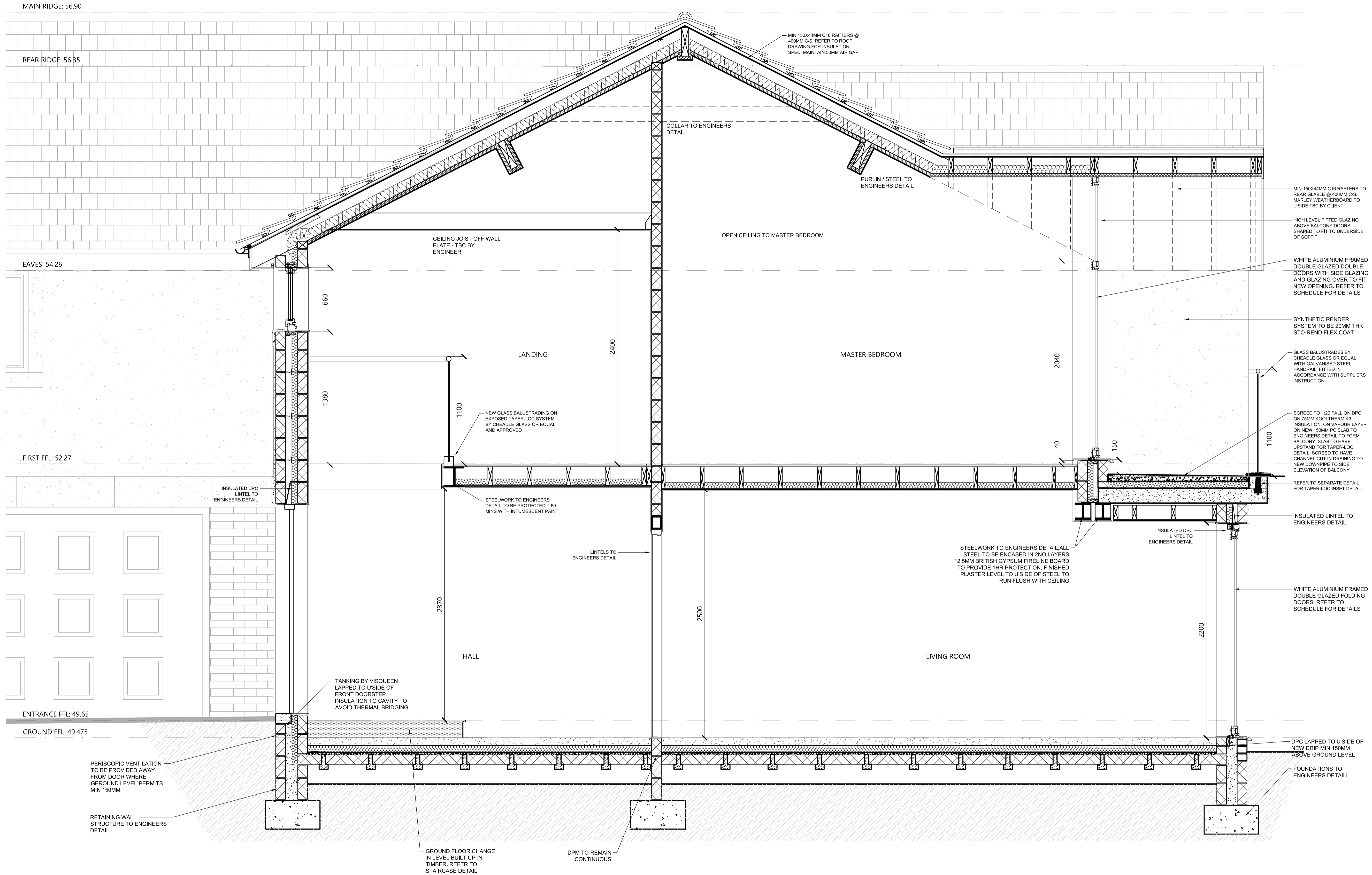
TYPICAL SECTION 5A HOUSE NO.5
